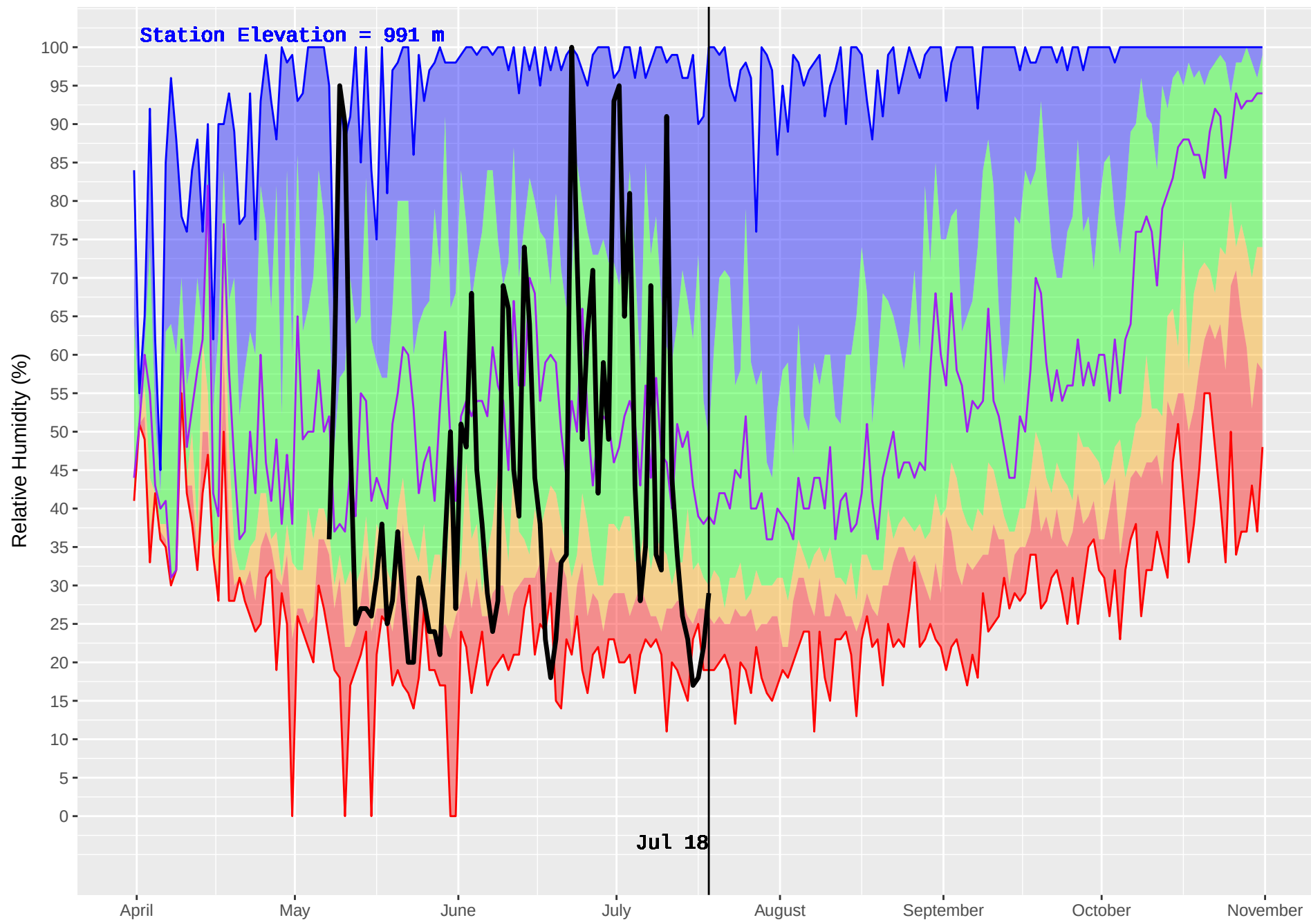
TROUT LAKE (387) : Historical (1987–2016) and Current (2018) Daily Relative Humidity
