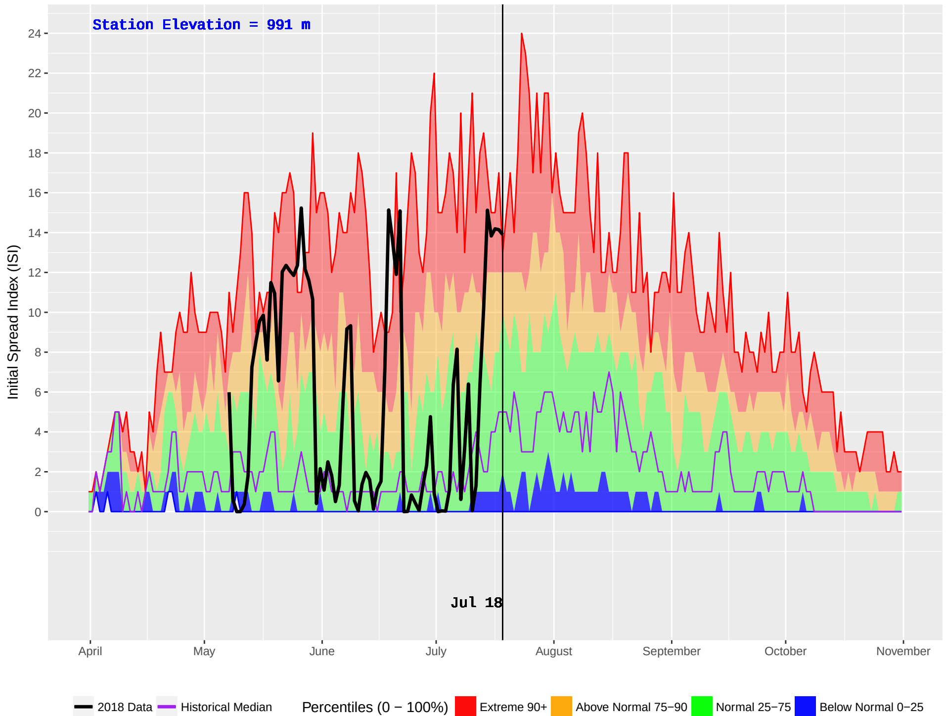
TROUT LAKE (387) : Historical (1987–2016) and Current (2018) Daily Initial Spread Index (ISI)
