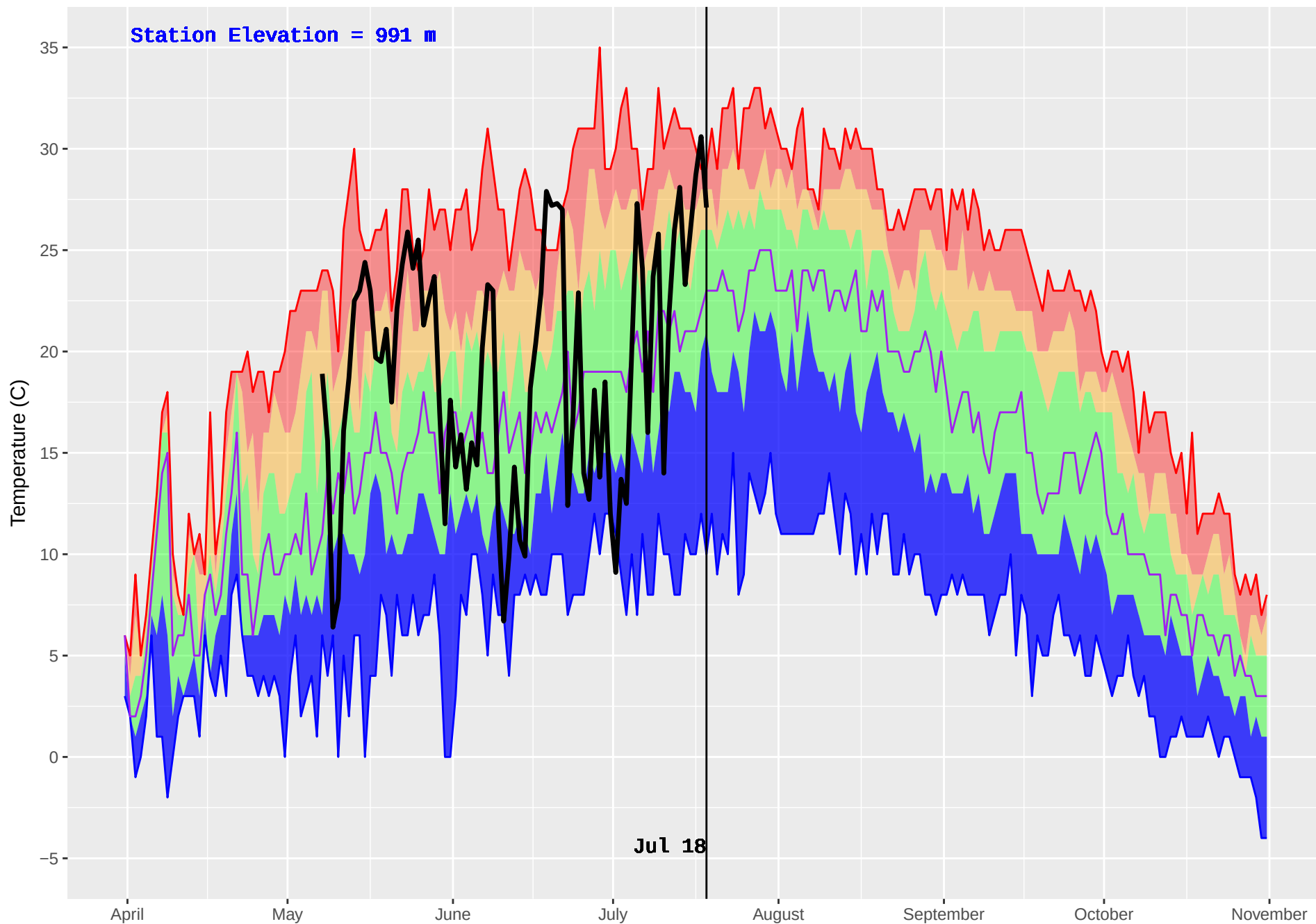
TROUT LAKE (387) : Historical (1987–2016) and Current (2018) Daily Temperature
