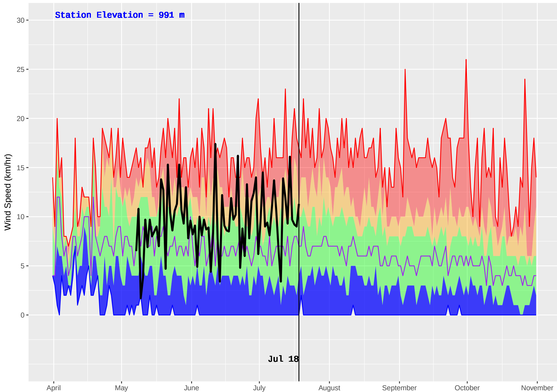
TROUT LAKE (387) : Historical (1987–2016) and Current (2018) Daily Wind Speed
